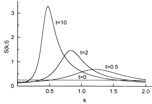
FIG. 1. Angle averaged structure factor S(k,t) vs k (in units of inverse lattice spacing) at early stages of decomposition of a model binary equiatomic square alloy, with NN effective pair interaction K^I = -0.5 .
